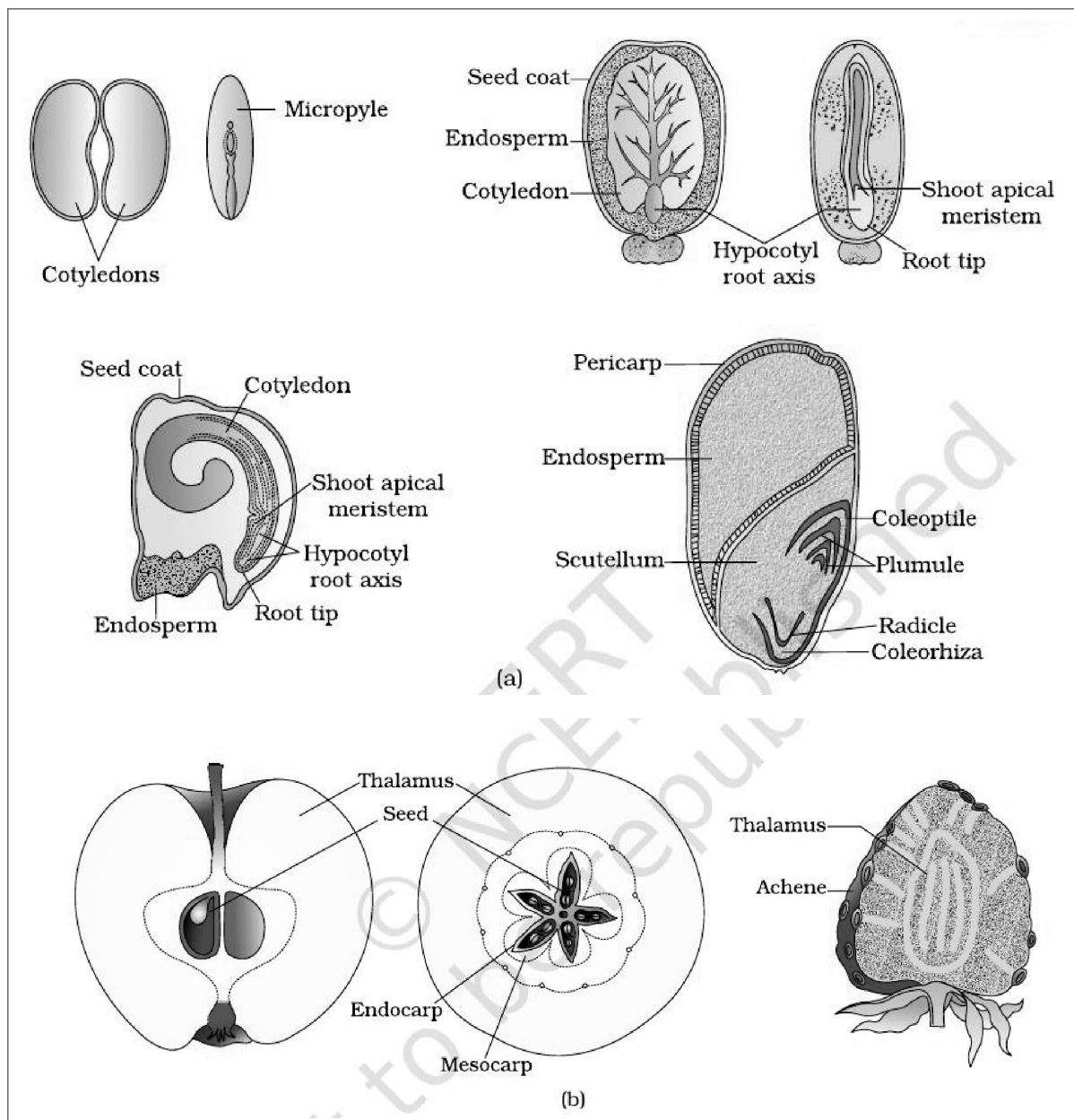
Fig. 1.15 — (a) Structure of some seeds. (b) False fruits of apple and strawberry. Labelled: cotyledons, micropyle, seed coat, endosperm, hypocotyl root axis, shoot apical meristem, root tip, scutellum, coleoptile, plumule, radicle, coleorhiza, pericarp, thalamus, seed, endocarp, mesocarp, achene.
